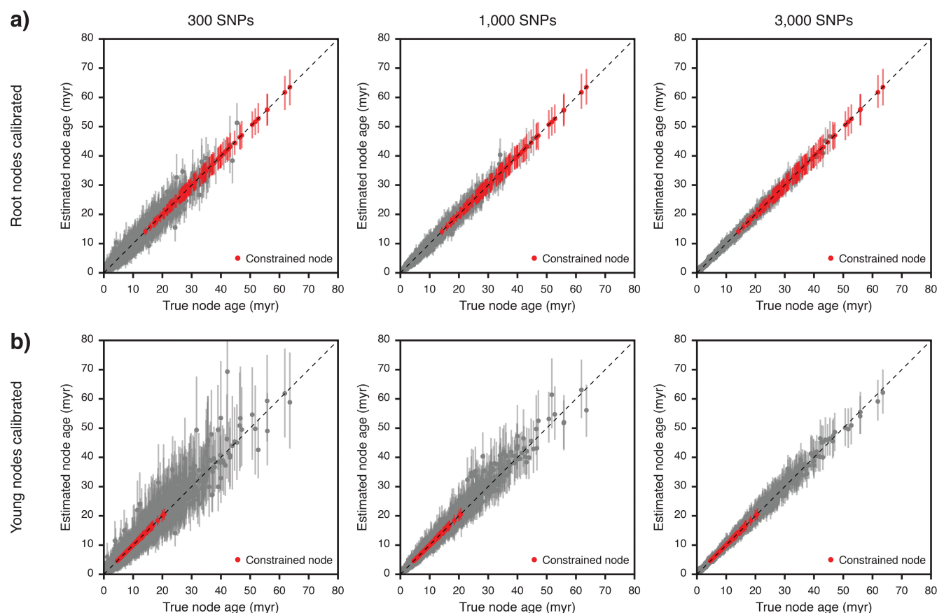
FIGURE 1. Comparison of true and estimated node ages (experiment 1). Results are based on 100 species trees and 300 to 3 000 SNPs generated per species tree. a) Node ages estimated with an age constraint on the root. b) Node ages estimated with an age constraint on a node that is approximately a third as old as the root. Mean age estimates of constrained and unconstrained nodes are marked with red and gray circles, respectively, and vertical bars indicate 95% HPD intervals.
